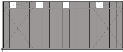
Right Elevation (External)
